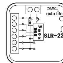
STEROWNIK LED RGBW SLR-22
