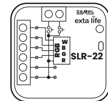
STEROWNIK LED RGBW SLR-22
